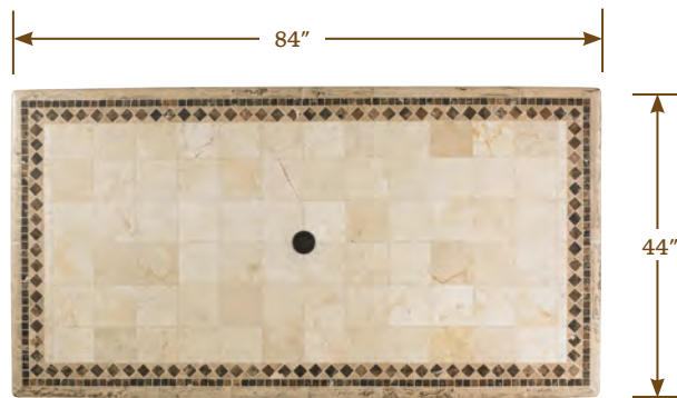
3160-876ST 84 x 44 in. Travertine and Marble Top 84W x 44D x 1.5H in.
