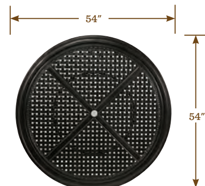
3190-870CT Sedona 54 in. Cast Aluminum Top 54 dia. x 2.25H in.
